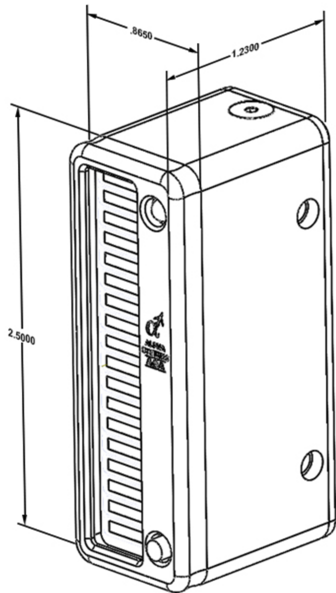
Falcon display technical drawing with dimensions
